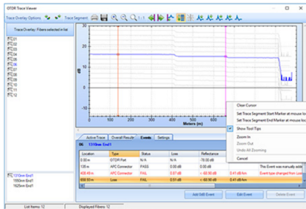
Setting span event parameters using LinkWare PC
